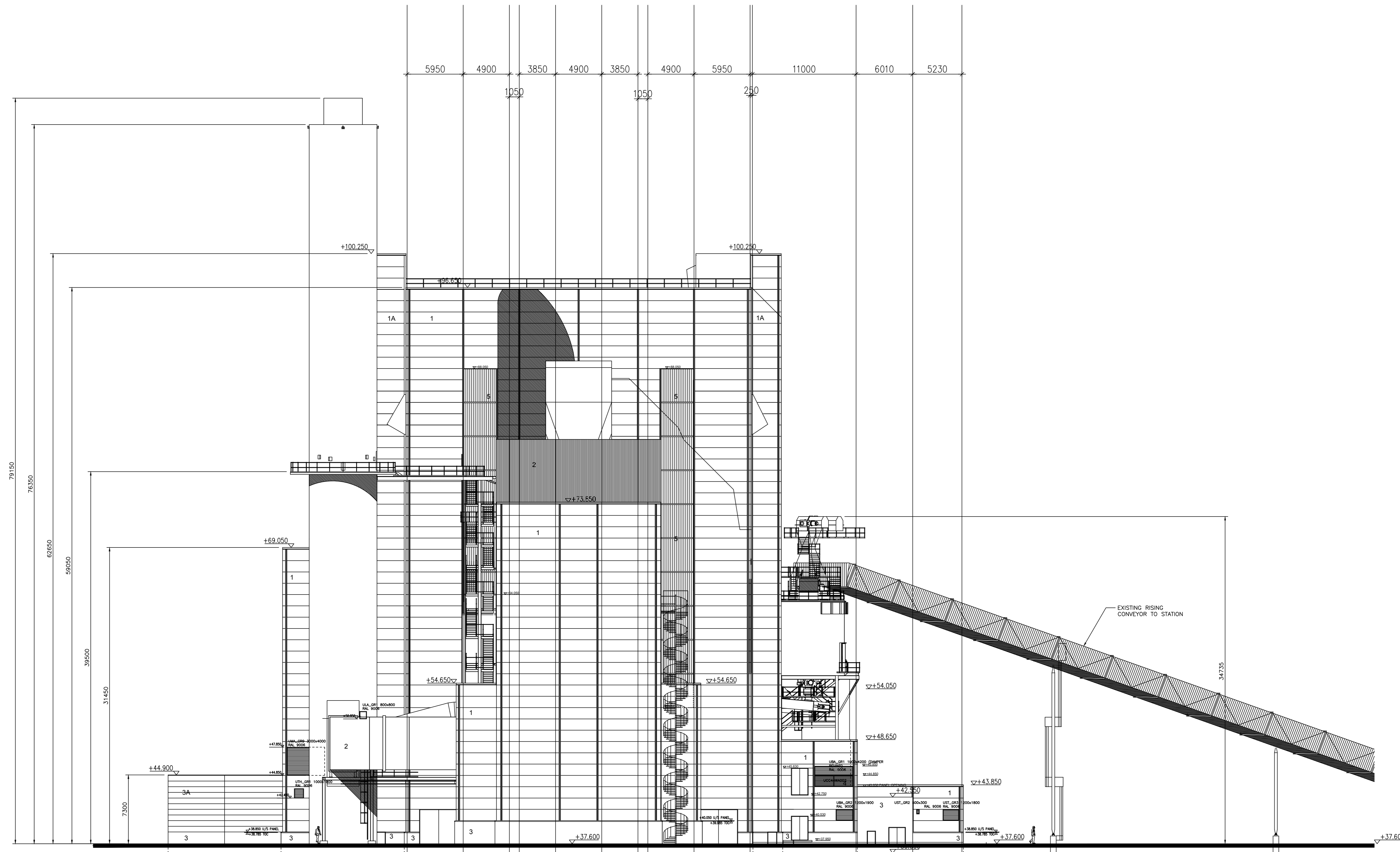
EAST ELEVATION
